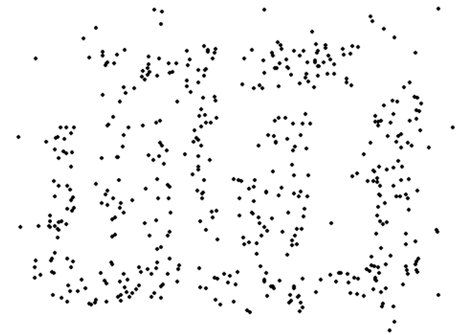
500 Points
