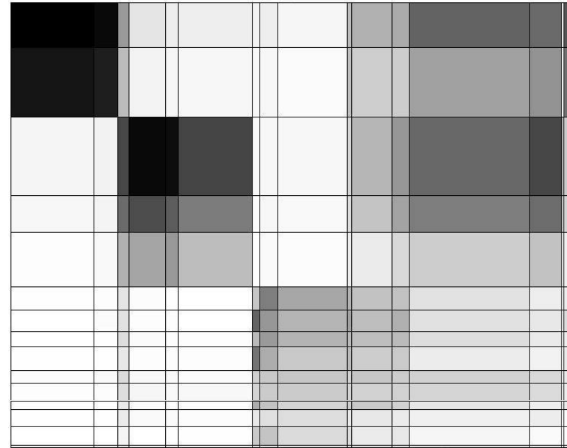
After clustering
