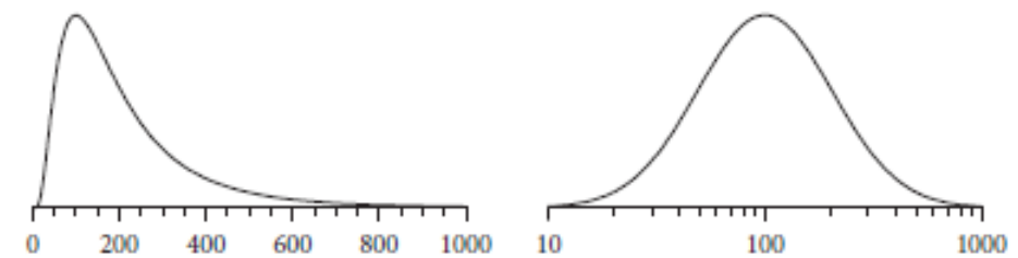
Figure 11.2. Lognormal distribution.
