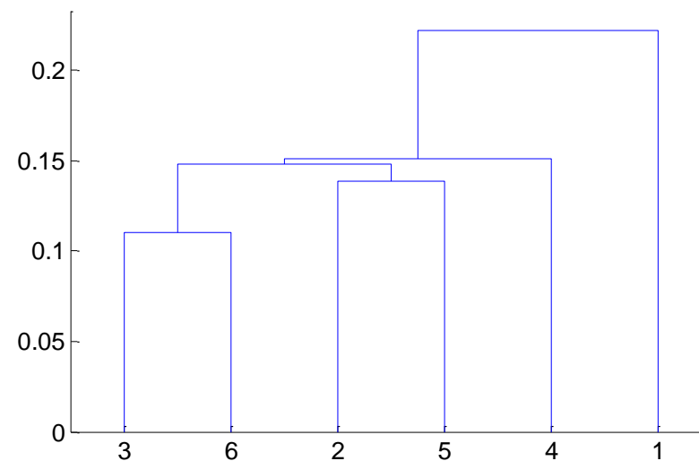
Dendrogram
