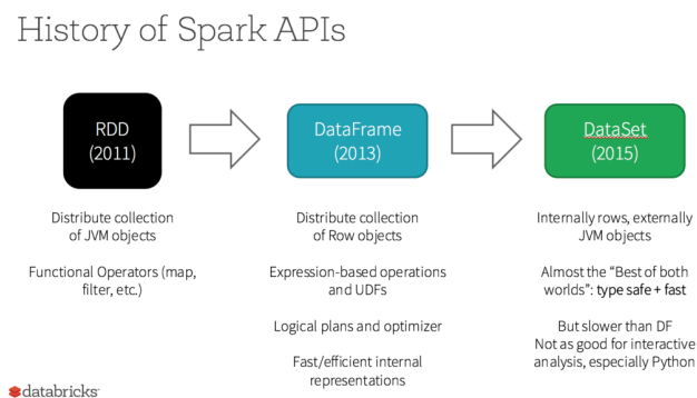
Figure 1. Evolution of Spark APIs [databr23].
