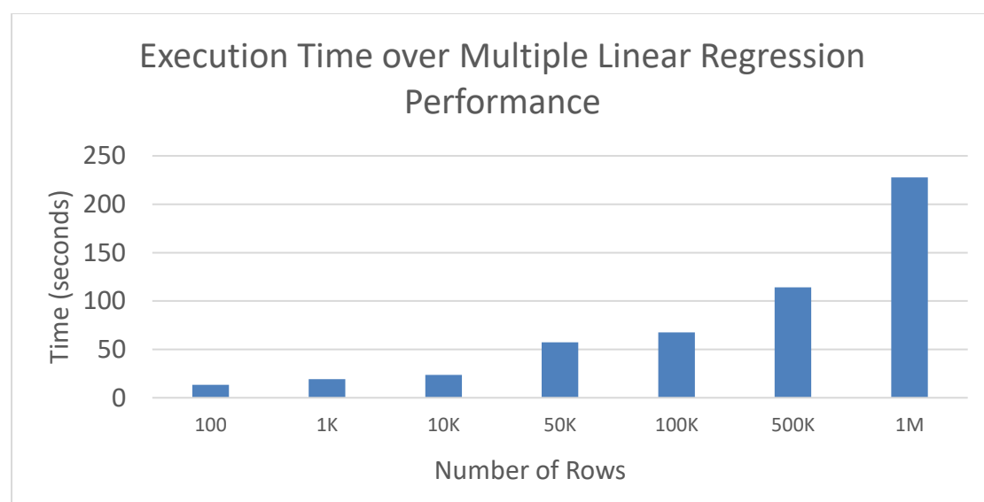
Figure 18. Bar chart showing how the number of rows affects the execution time of Multiple Linear Regression.
