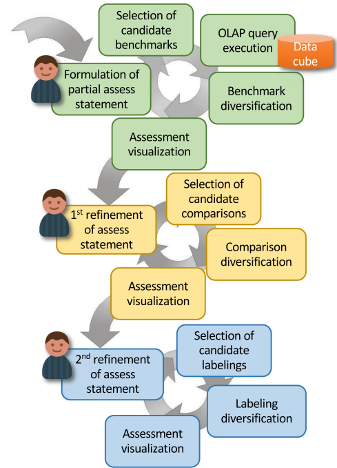
Fig. 2. Functional view of the progressive refinement process.
