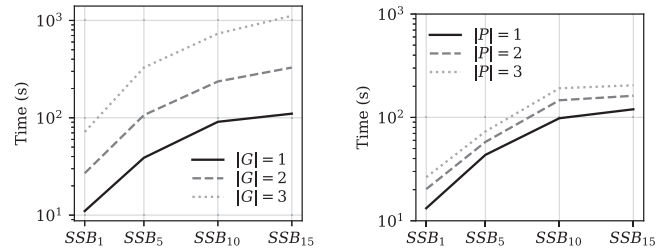
Fig. 7. Times for computing an assessment with parent (left) and sibling (right) benchmarks in auto-complete mode.
