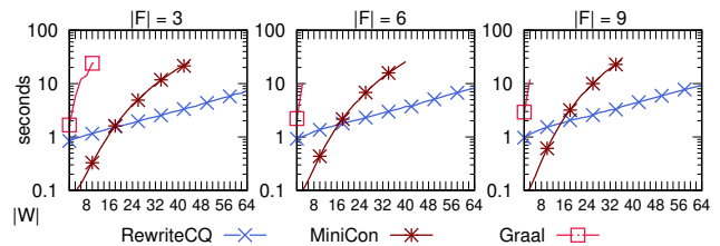
Fig. 3: Runtime evolution w.r.t. the number of wrappers ( |W| ) and alternative approach under comparison. Missing points denote that the execution of the alternatives timed out.
