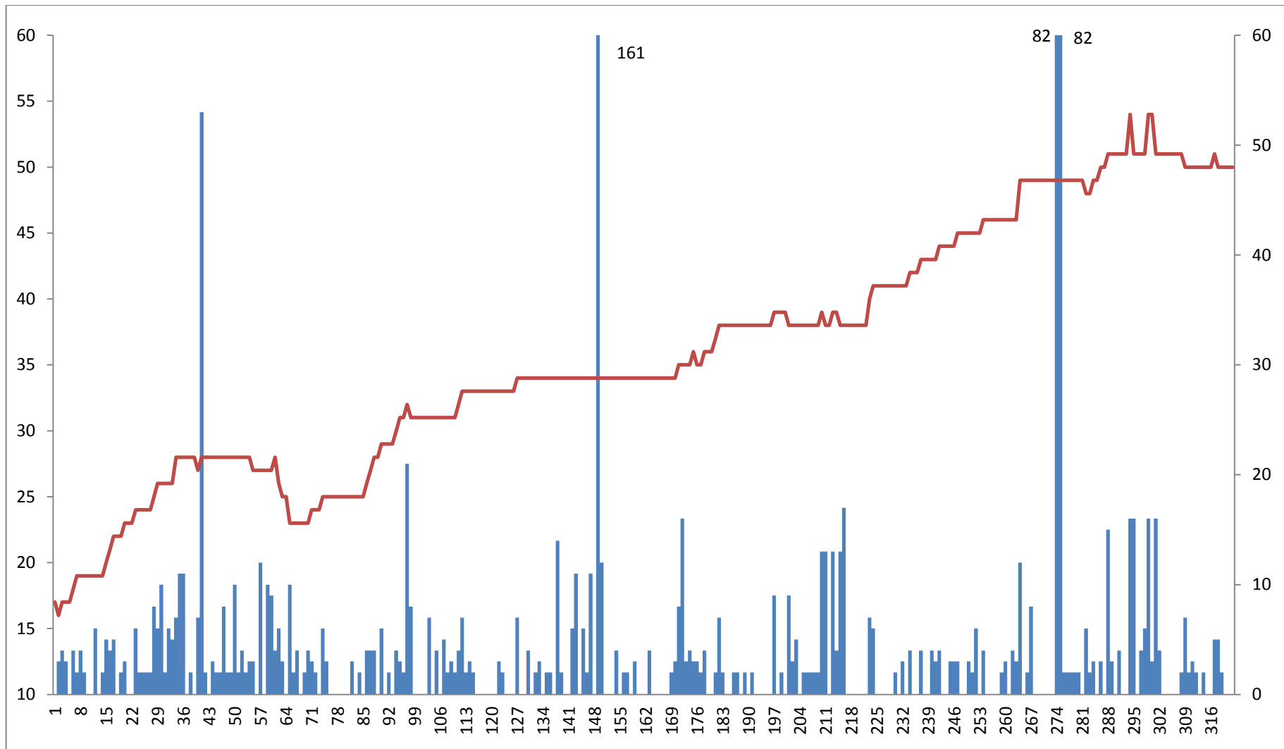
a) Changes compared with schema size for MediaWiki
