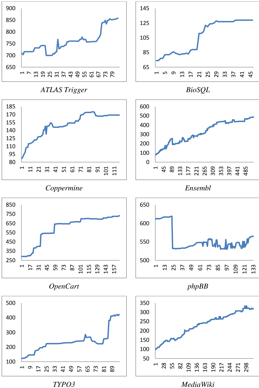
Figure 4.6 A comparative presentation of schema size per version, expressed as the number of attributes, for the studied database schemata
