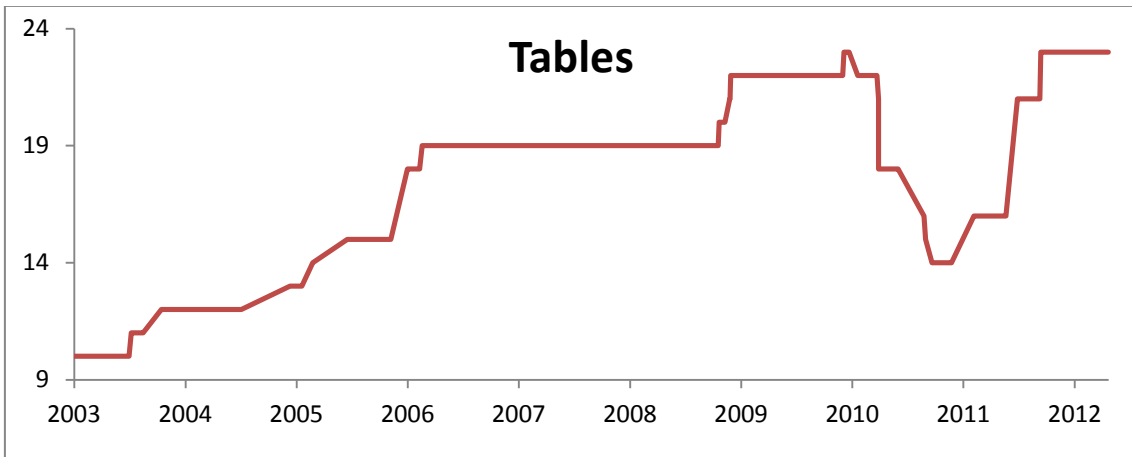
b) Number of Tables for TYPO3
