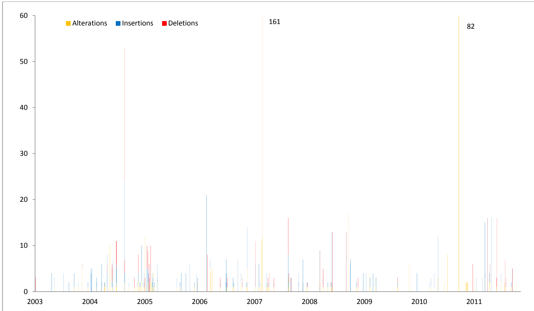
a) Changes Breakdown over Time for MediaWiki
