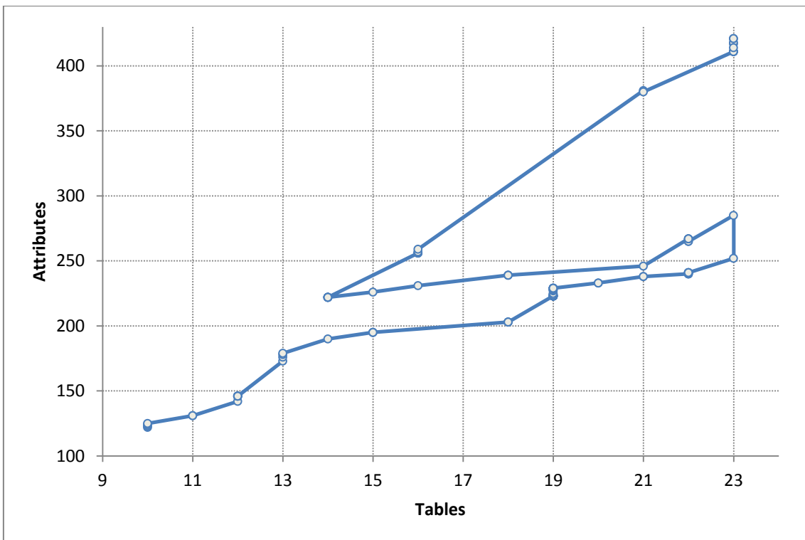
b) Timeline for TYPO3
