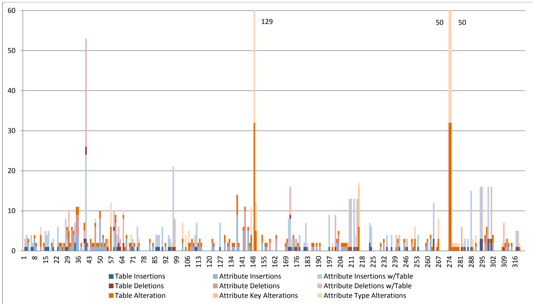
b) Changes Breakdown over Version ID for MediaWiki
