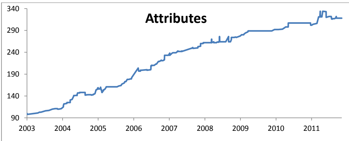
c) Number of Attributes for MediaWiki
