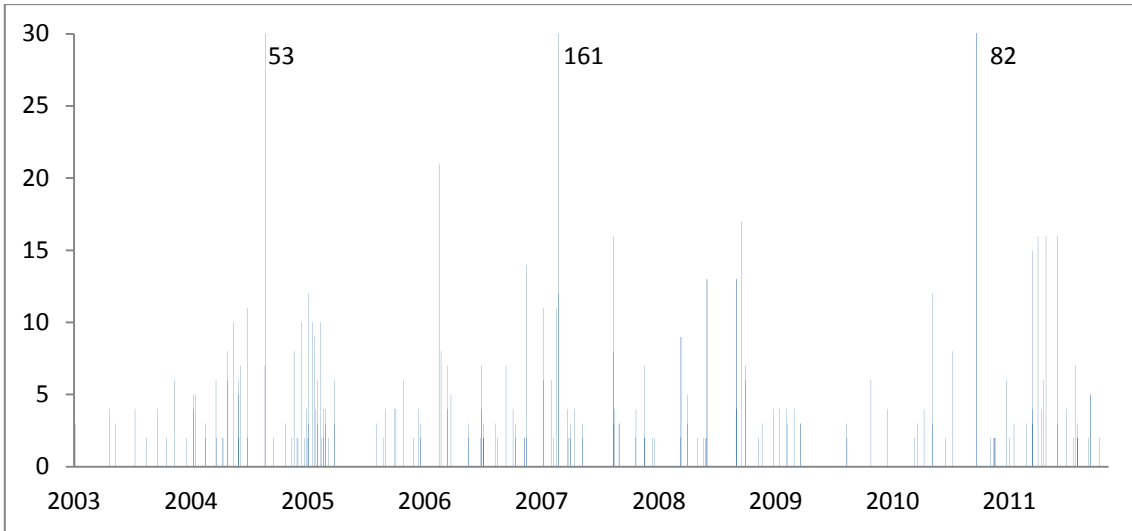
a) Changes Heartbeat over Time for MediaWiki
