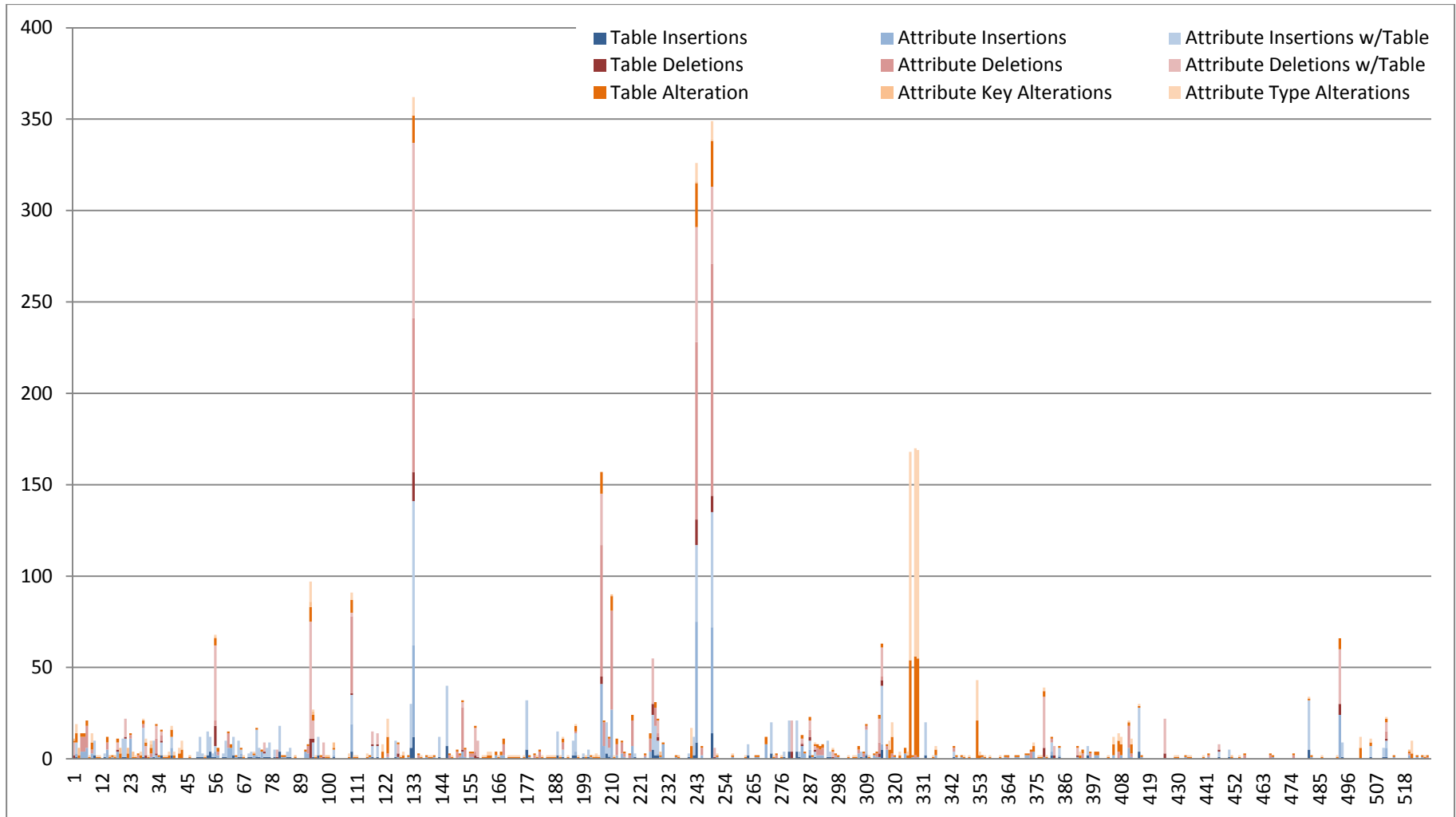
b) Changes Breakdown over Version ID for Ensembl
