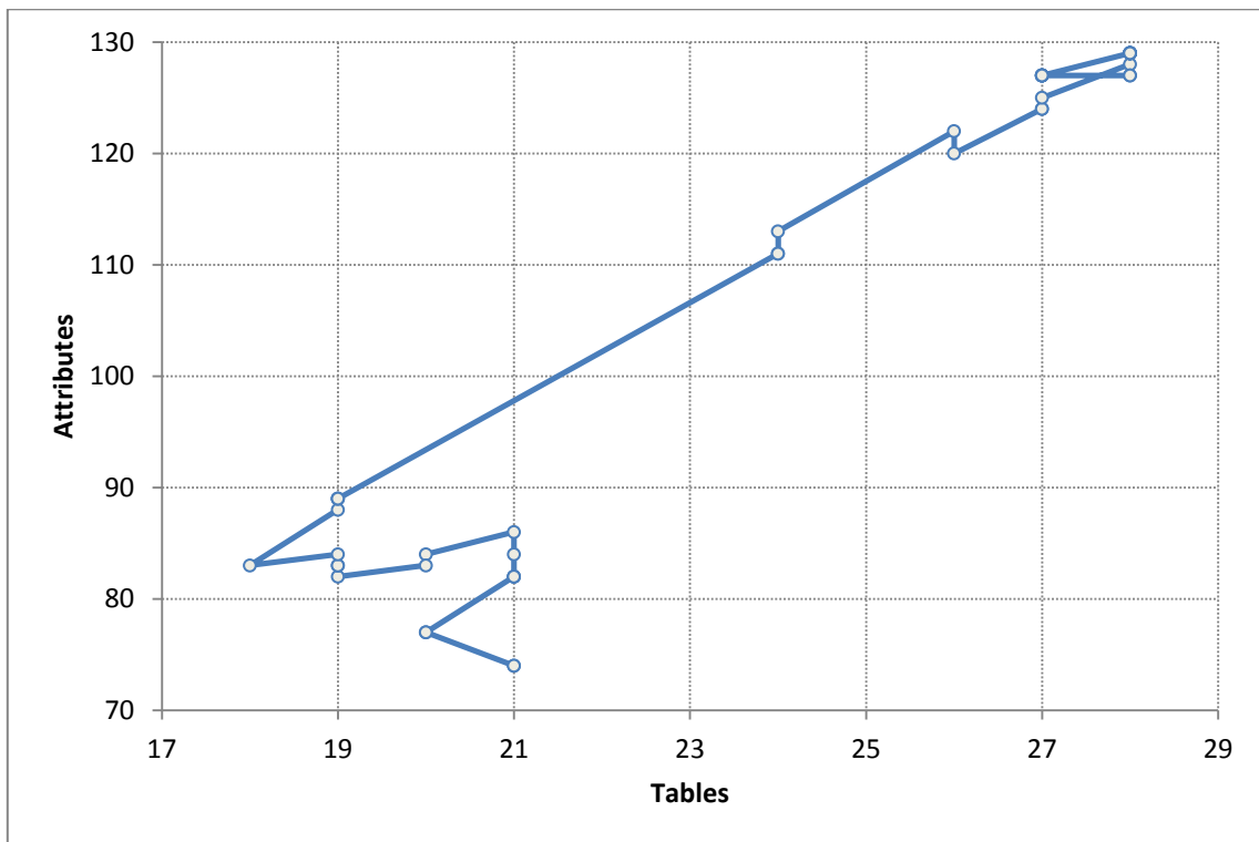
b) Timeline for BioSQL
