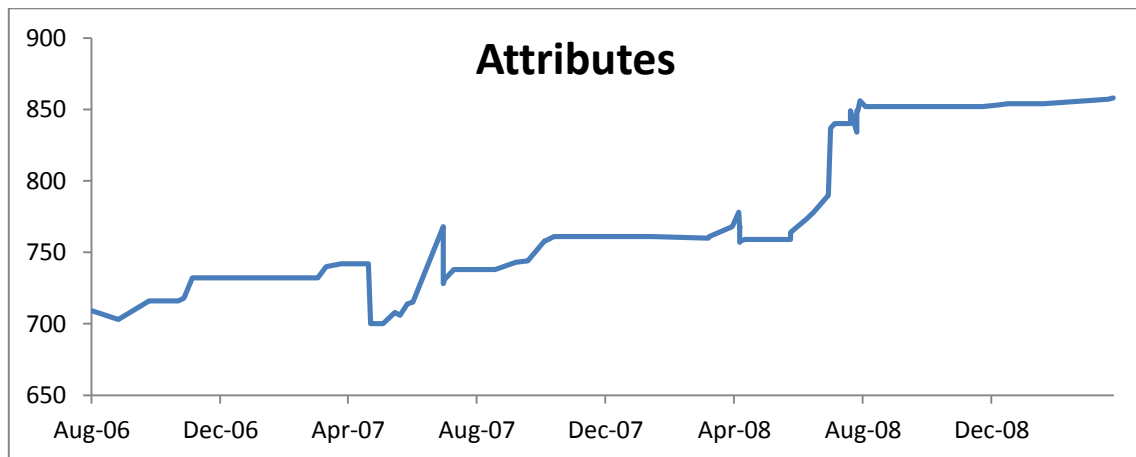
c. Number of Attributes for ATLAS Trigger
