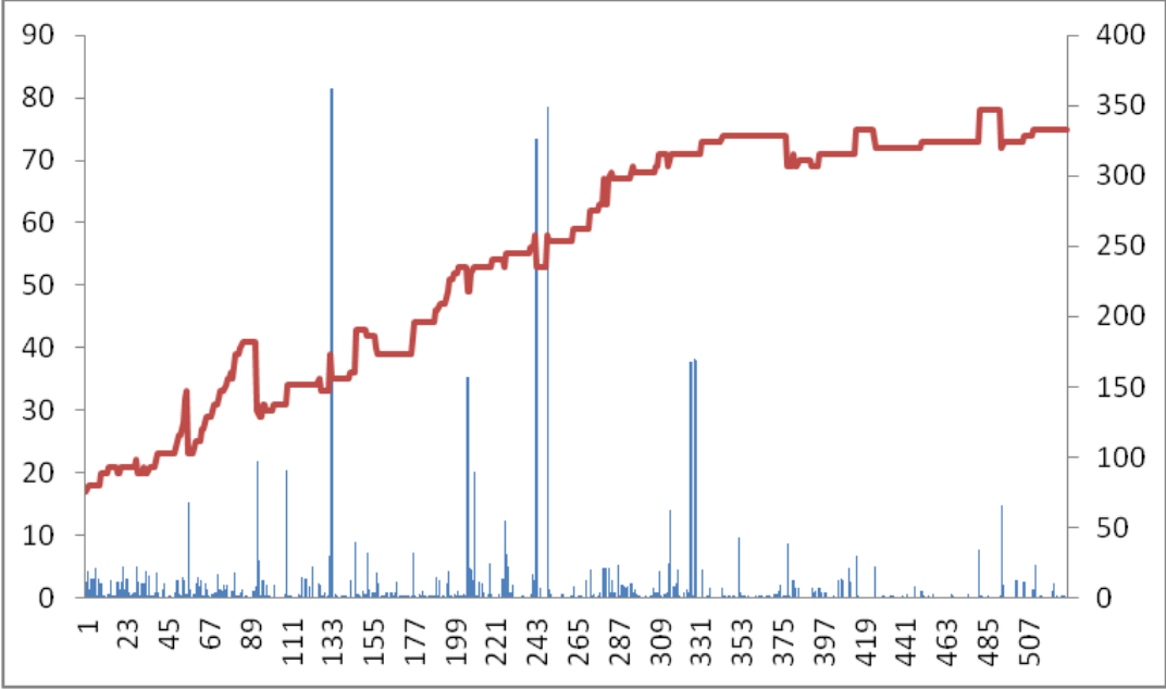
Figure 4.19 Ensemble’s combined heartbeat and schema size: age results in a decline of both activity and growth
