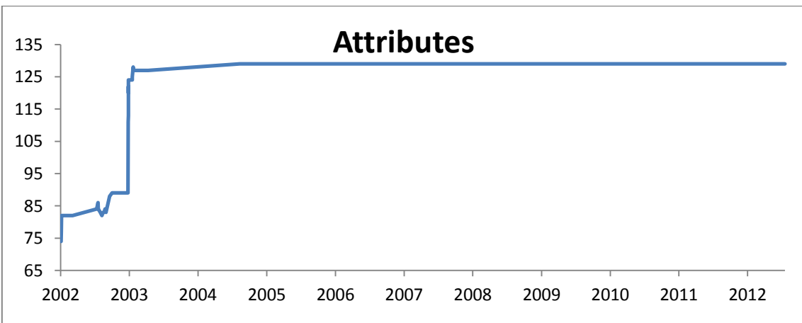
c) Number of Attributes for BioSQL
