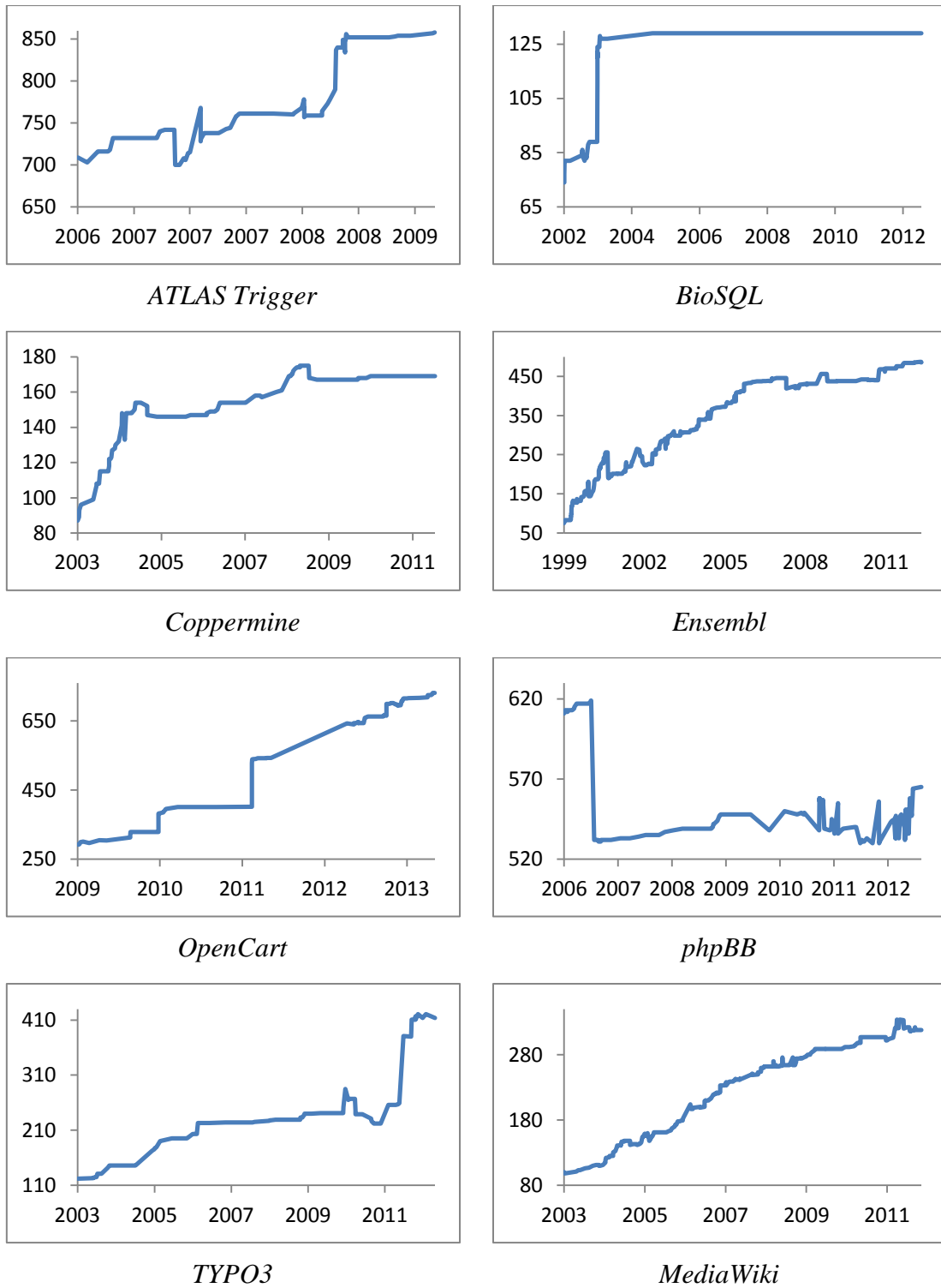
Figure 4.4 A comparative presentation of schema size per version over time, expressed as the number of attributes, for the studied database schemata
