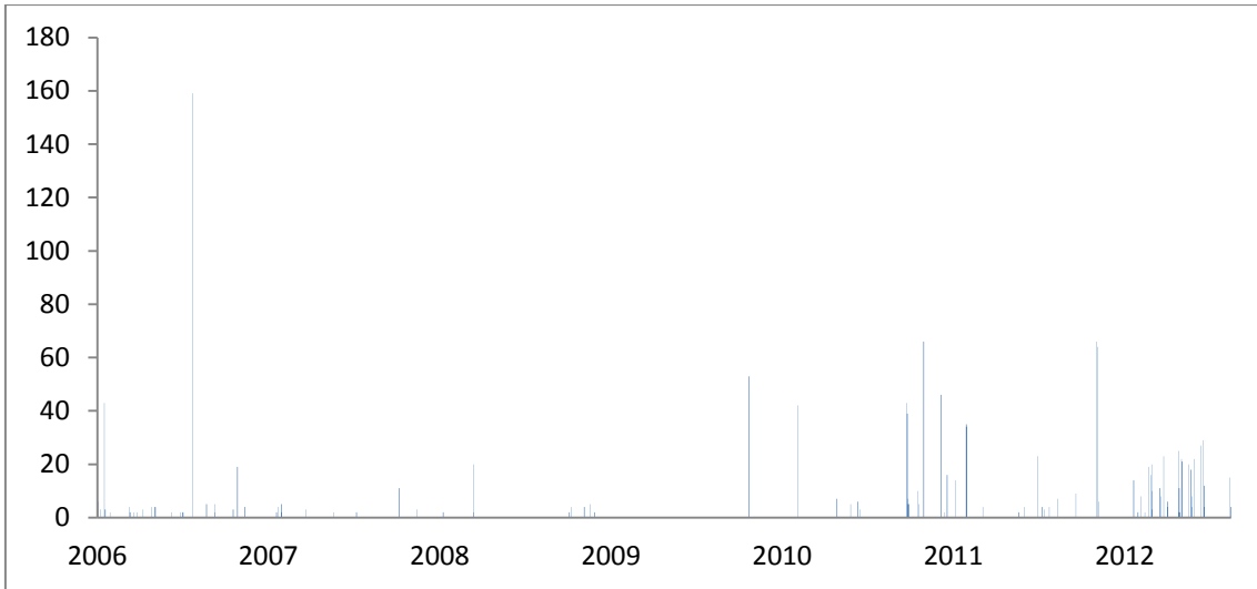
a) Changes Heartbeat over Time for phpBB
