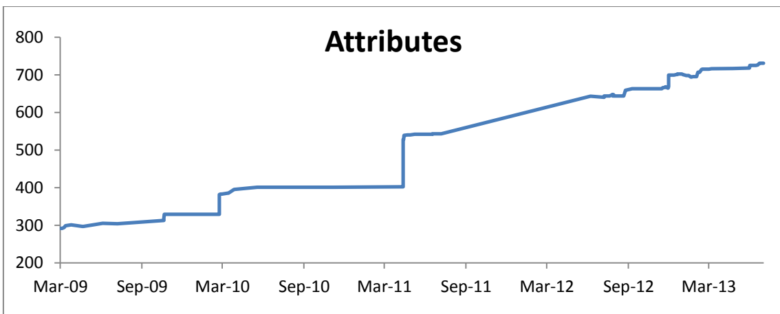
c) Number of Attributes for OpenCart
