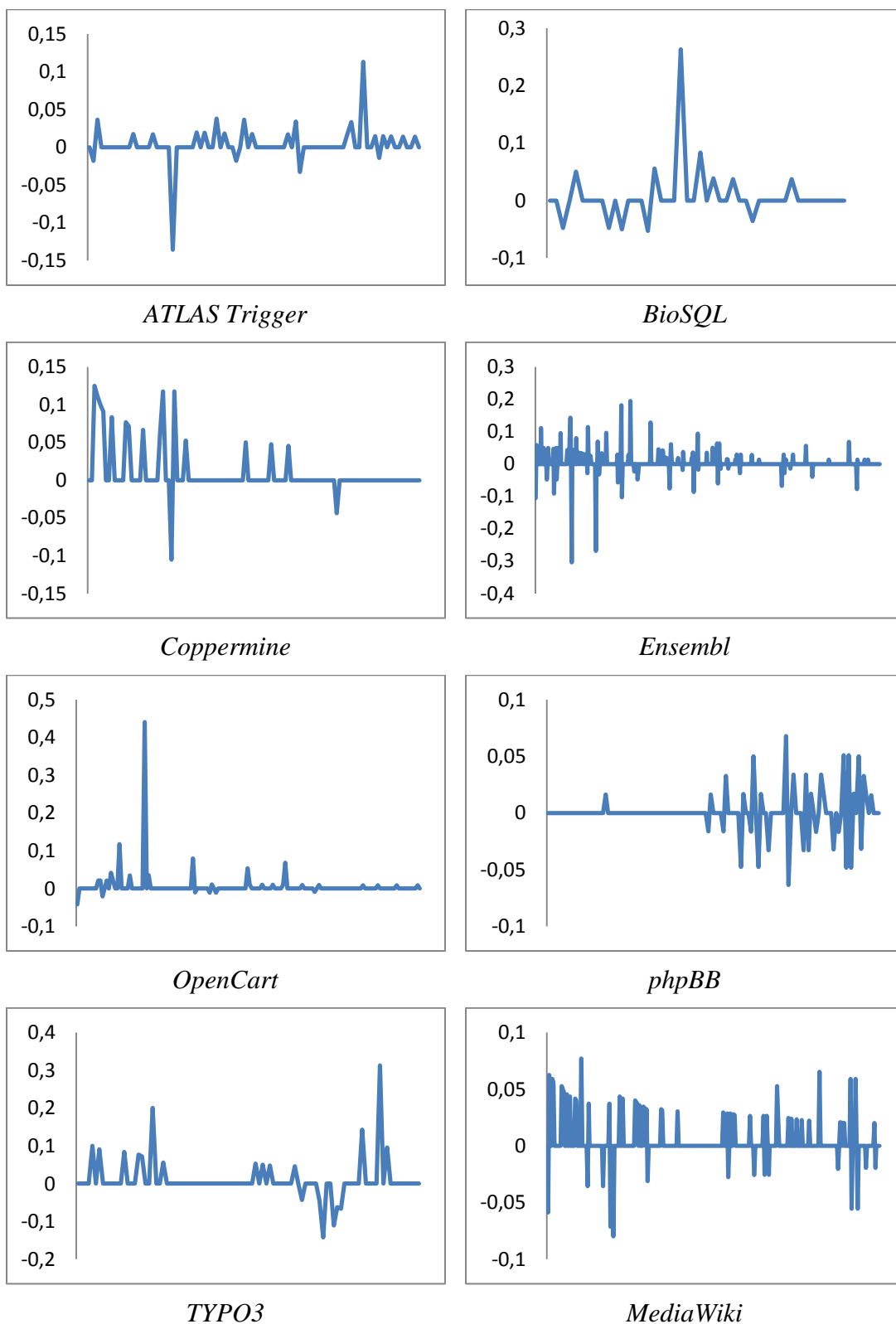
Figure 4.14 A comparative presentation of growth ratio for the studied database schemata
