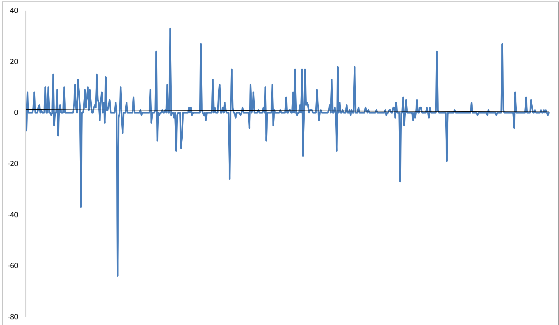
Figure 4.13 Zoomed growth (in number of attributes) for MediaWiki over version ID
