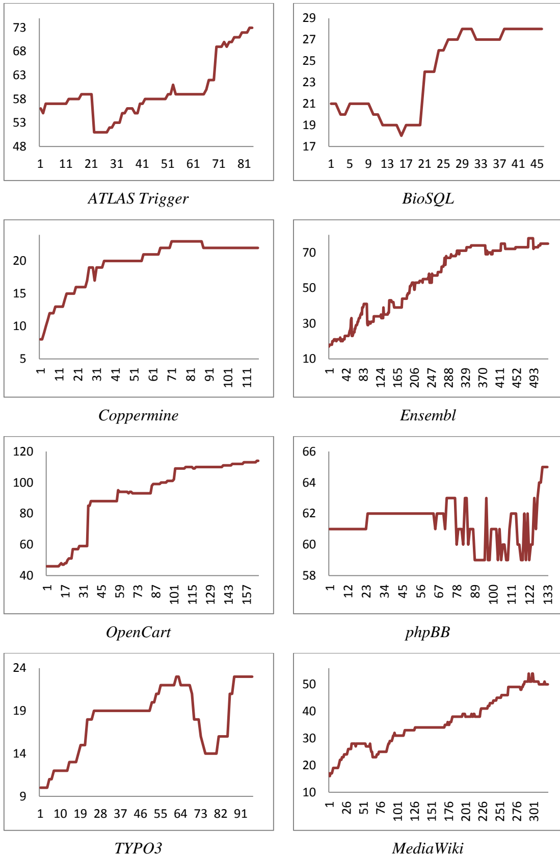
Figure 4.5 A comparative presentation of schema size per version, expressed as the number of relations, for the studied database schemata
