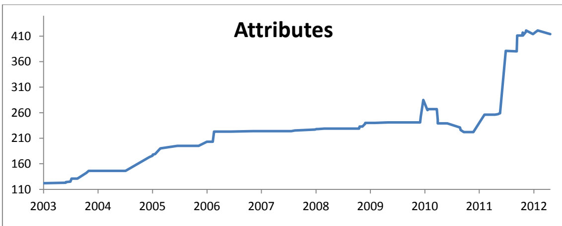
c) No. of Attributes for TYPO3
