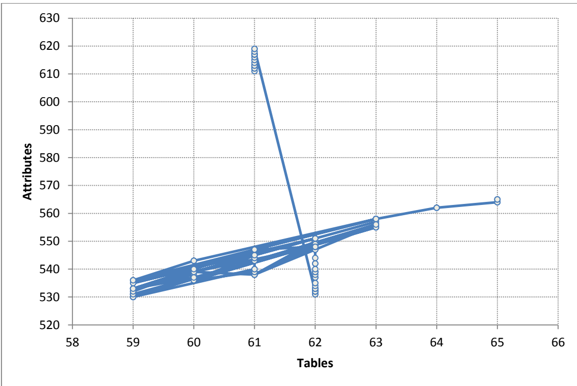
b) Timeline for phpBB
