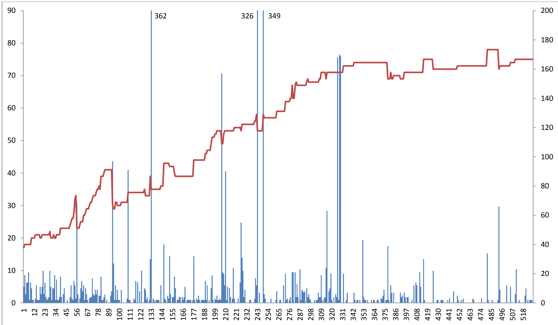
a) Changes compared with schema size for Ensembl
