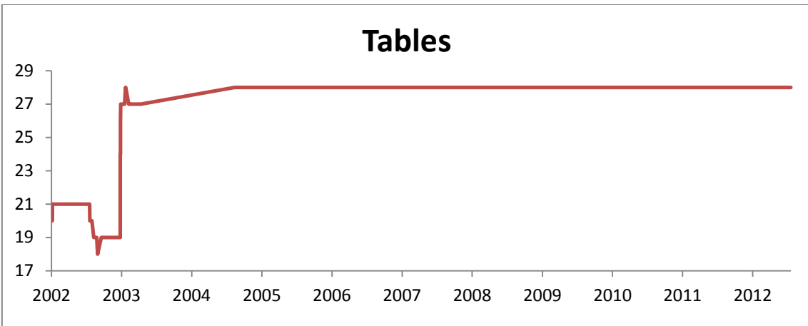
b) Number of Tables for BioSQL
