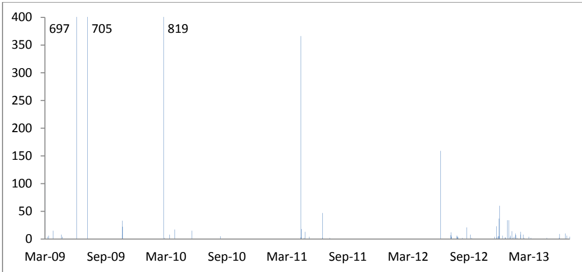
a) Changes Heartbeat over Time for OpenCart
