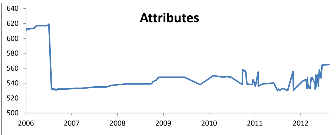
c) Number of Attributes for phpBB
