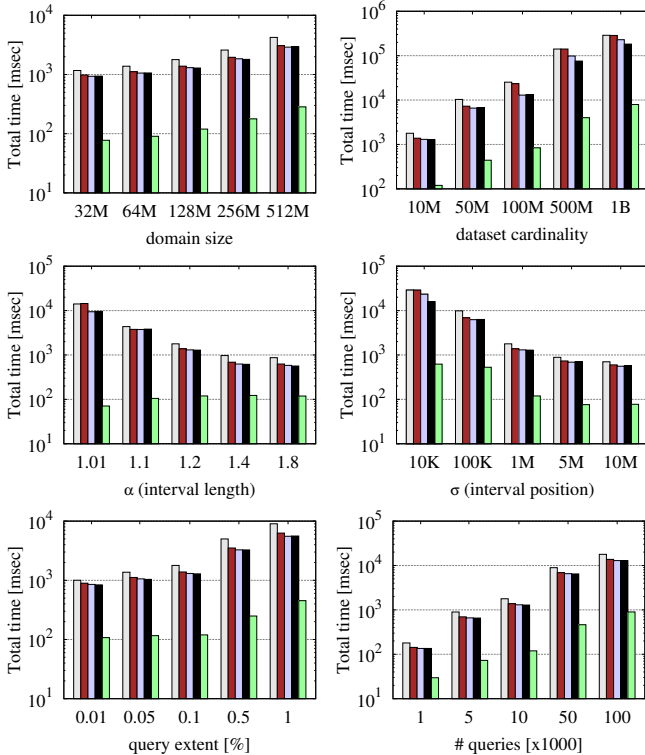
Fig. 7: Batch processing selection queries (synthetic datasets)
