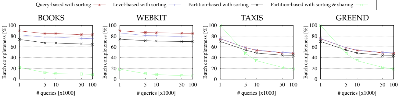
Fig. 8: Impact of batch processing - lower numbers better; default query extent 0.1%
