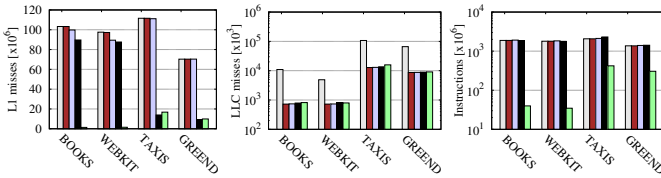
Fig. 6: Advanced stats; defaults 0.1% extent, 10K queries
