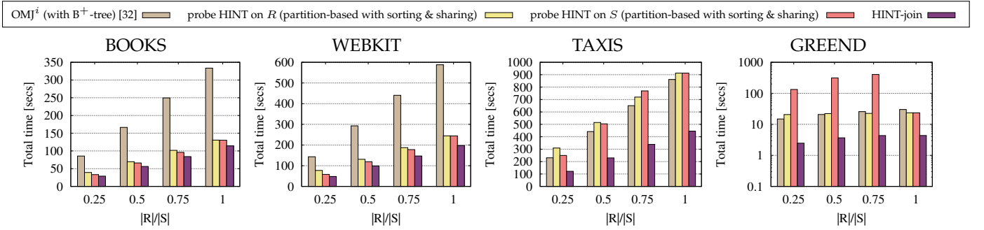
Fig. 11: Joining indexed inputs
