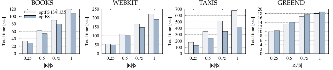
Fig. 10: Joining unindexed inputs
