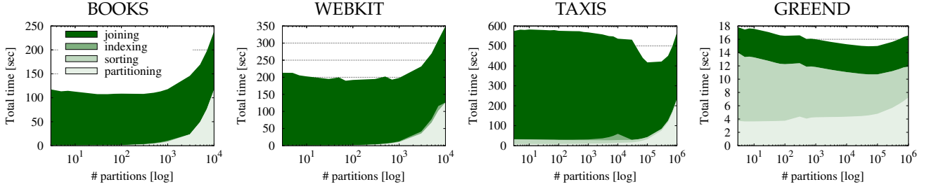
Fig. 9: Determining the optimal partitioning granularity for optFS+, time breakdown
