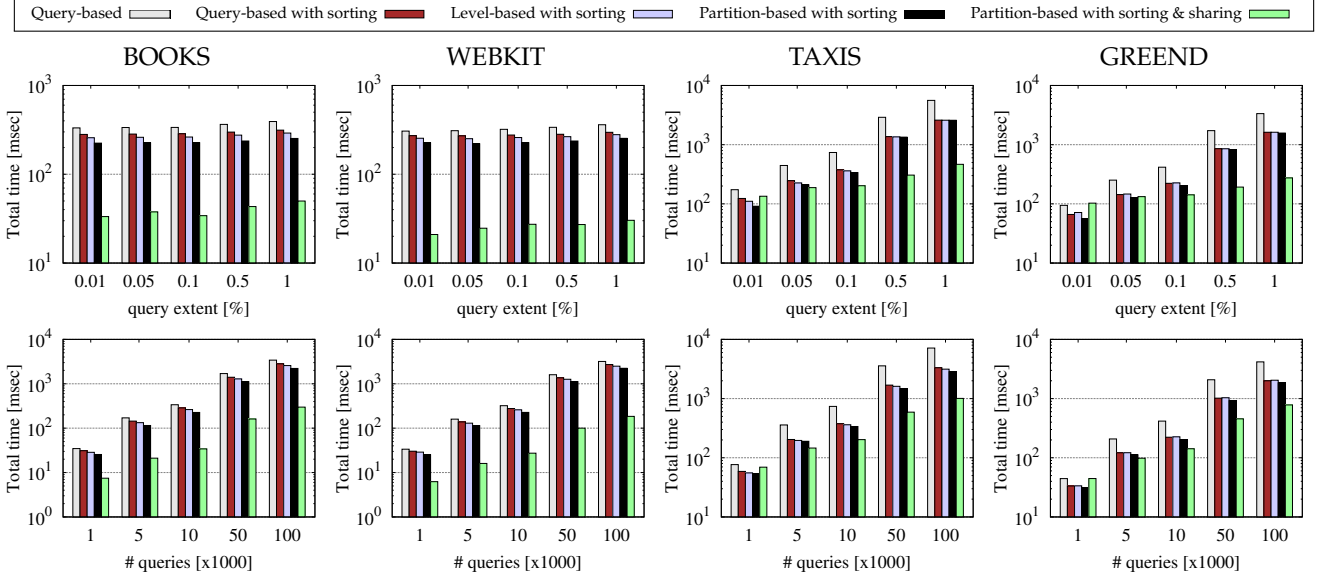
Fig. 5: Batch processing selection queries (real datasets)
