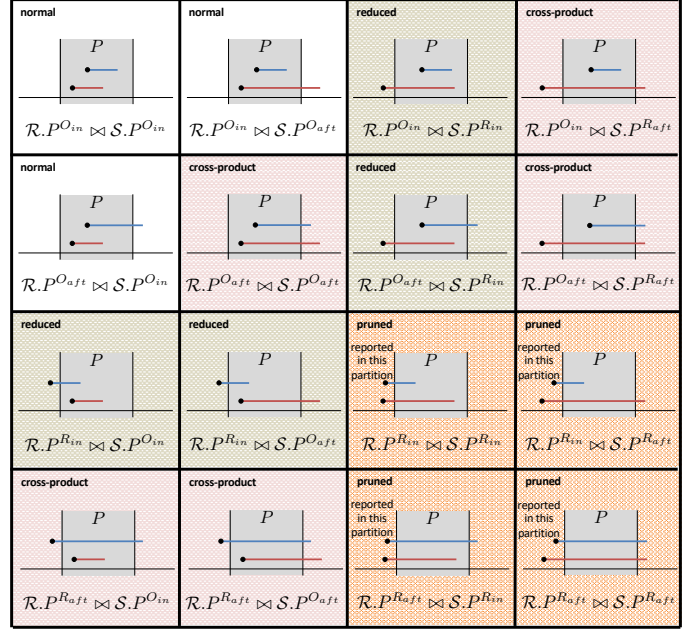
Fig. 4: Mini-joins breakdown for partition-to-partition joins
