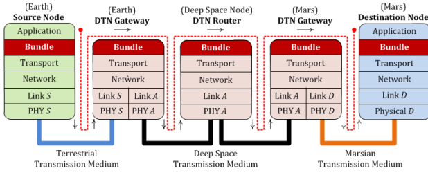
Fig. 12. DTN protocol stack communication diagram.
