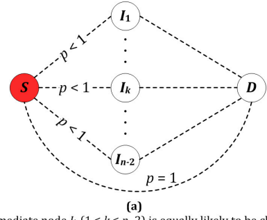
(a) Any intermediate node I_k (1 \leq k \leq n-2) is equally likely to be chosen by S except D to which the bundle is forwarded with probability 1.
