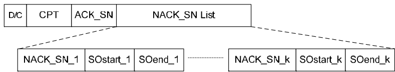
Figure 4.15: STATUS PDU format.
