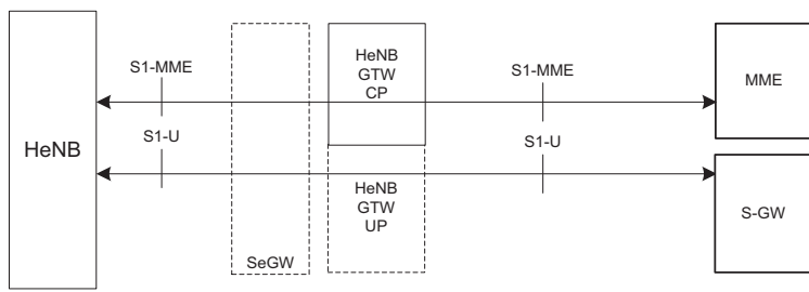
Figure 24.1: E-UTRAN HeNB logical architecture. Reproduced by permission of © 3GPP.
