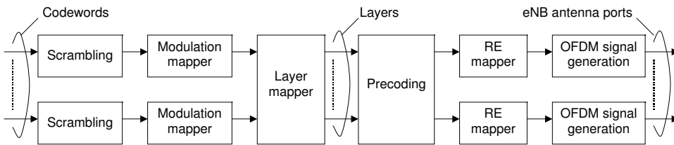
Figure 6.3: General signal structure for LTE downlink.
