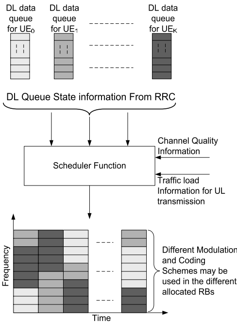
Figure 12.2: Generic view of a wideband resource scheduler.
