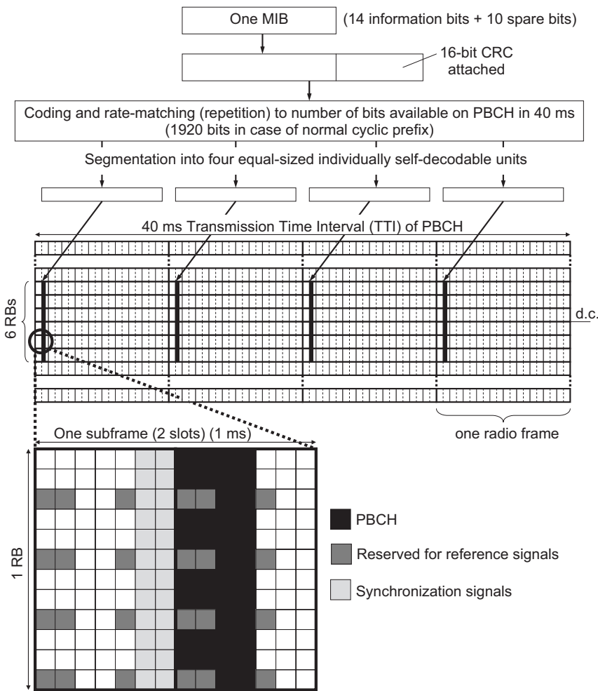
Figure 9.1: PBCH structure.
