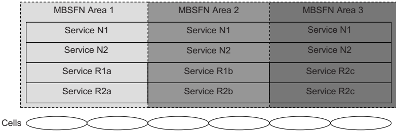
Figure 13.7: Example scenario without overlapping MBSFN areas.
