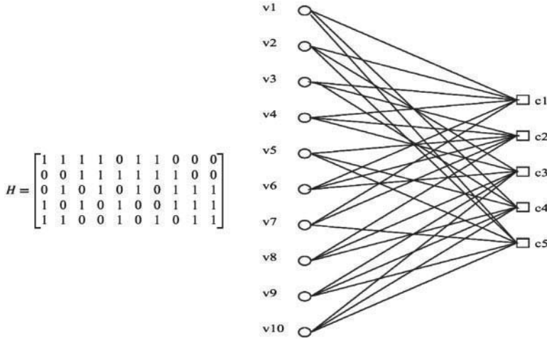
Figure 10.8: A Tanner graph representing the parity-check matrix of a (3, 6)-regular LDPC code C(10, 5) and its associated parity-check matrix H .
