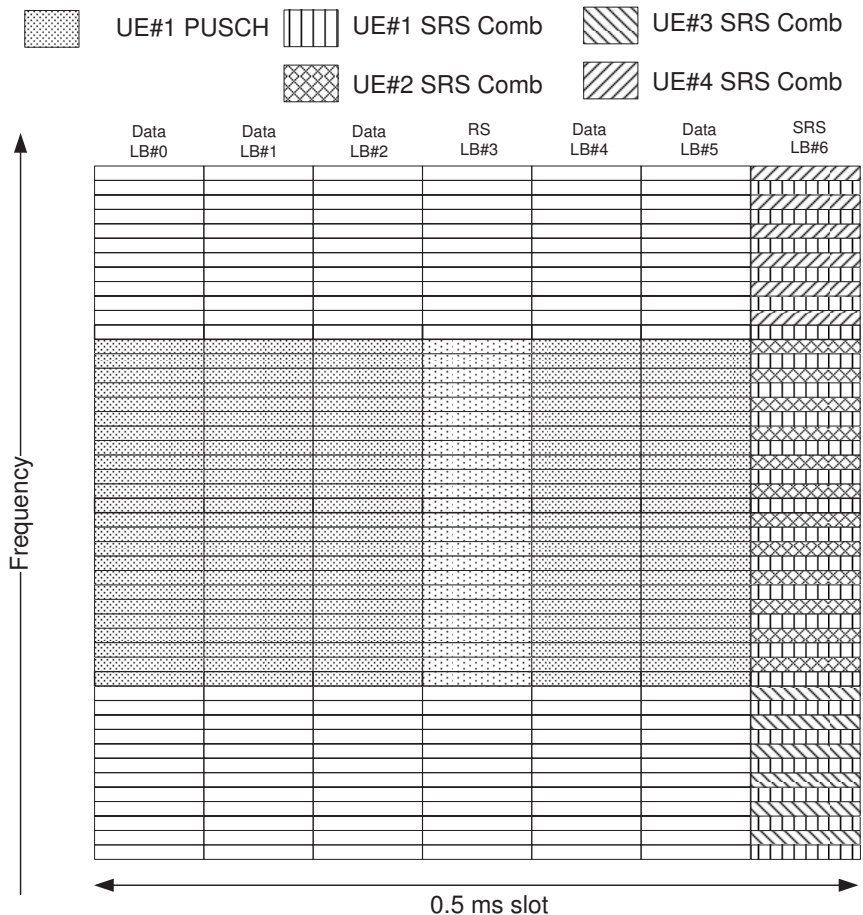
Figure 15.9: SRS symbol structure with RPF = 2.
