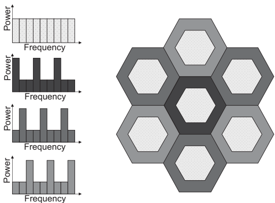
Figure 12.6: Partial frequency reuse.
