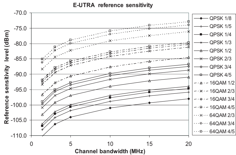
Figure 21.12: LTE UE reference sensitivity.
