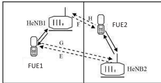
Figure 24.6: Femto/femto interference scenarios.
