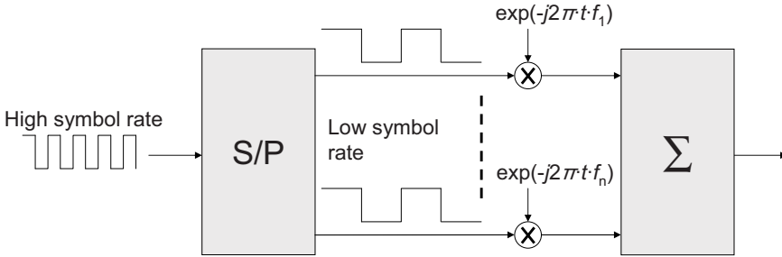
Figure 5.2: Serial-to-Parallel (S/P) conversion operation for OFDM.
