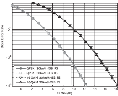
Figure 15.5: Demodulation performance comparison for Long Block RS and Short Block RS structure. Code rate r = 1/2 , GSM Typical Urban (TU) channel model, 30 km/h, 2 GHz carrier frequency.
