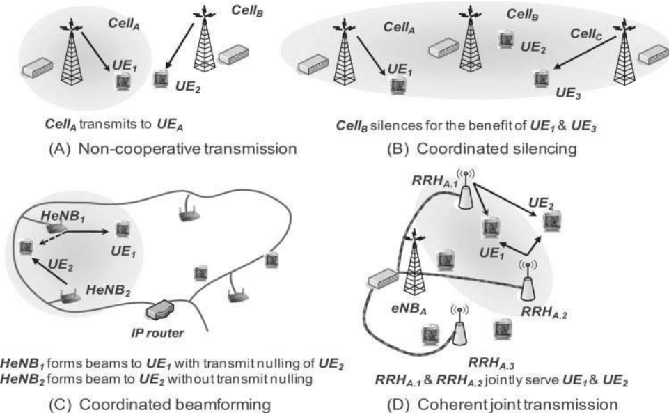
Figure 29.11: Downlink transmission schemes: (A) non-cooperative transmission; (B) coordinated scheduling; (C) coordinated beamforming; (D) coherent joint transmission.
