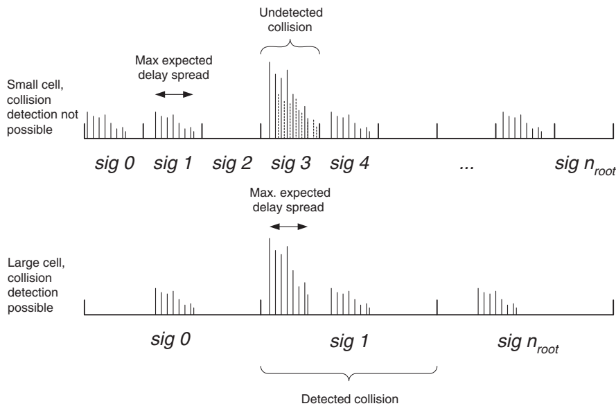
Figure 17.29: Collision detection.
