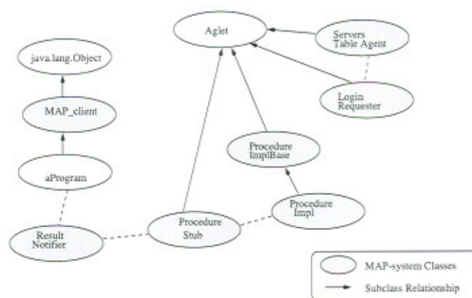
Figure 3: The Client Object Model
