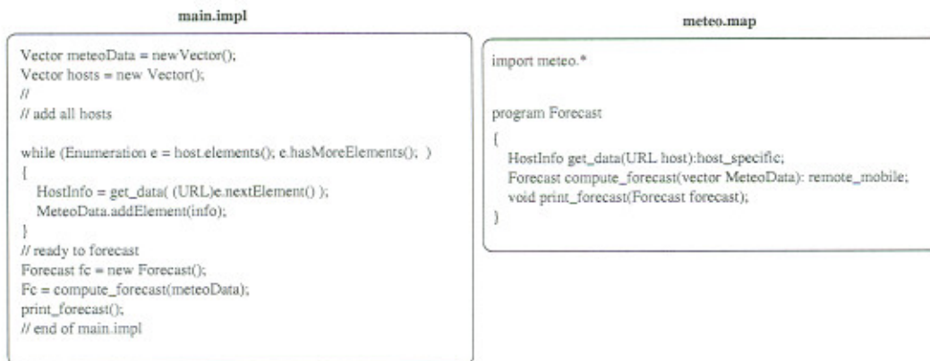
Figure 5: MAP Example.
