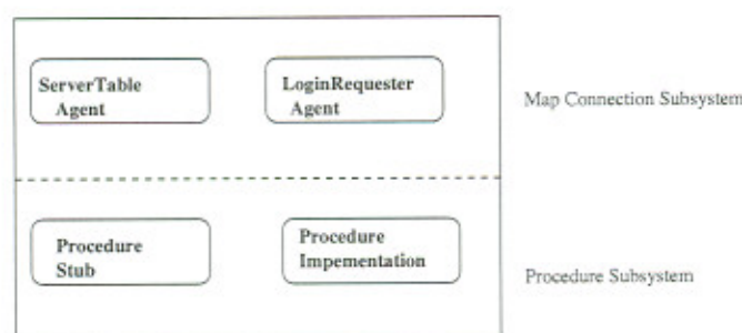
Figure 2: The Components of a MAP Client.
