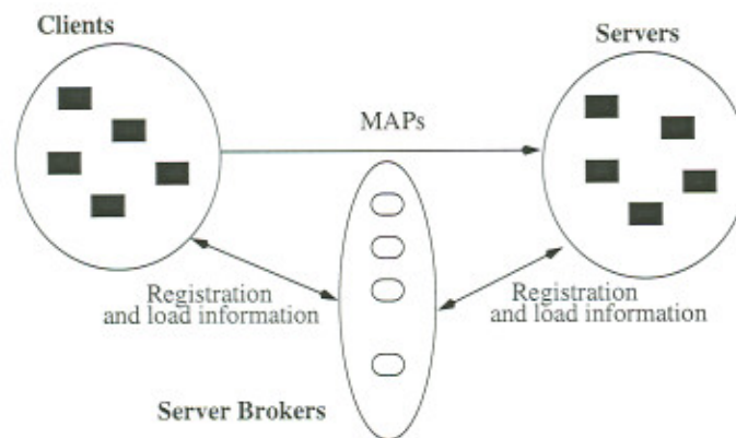
Figure 1: MAP's Architecture.
