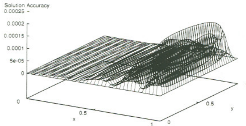
Figure 18: Problem 6: Accuracy of the FEM solution at the training points.
