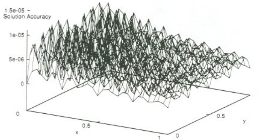
Figure 17: Problem 5: Accuracy of the FEM solution at the test points.
