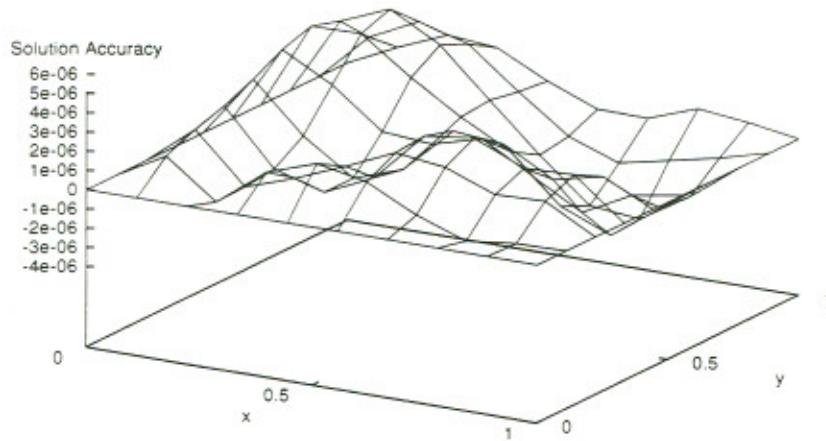
Figure 14: Problem 7: Accuracy of the computed solution at the training points.
