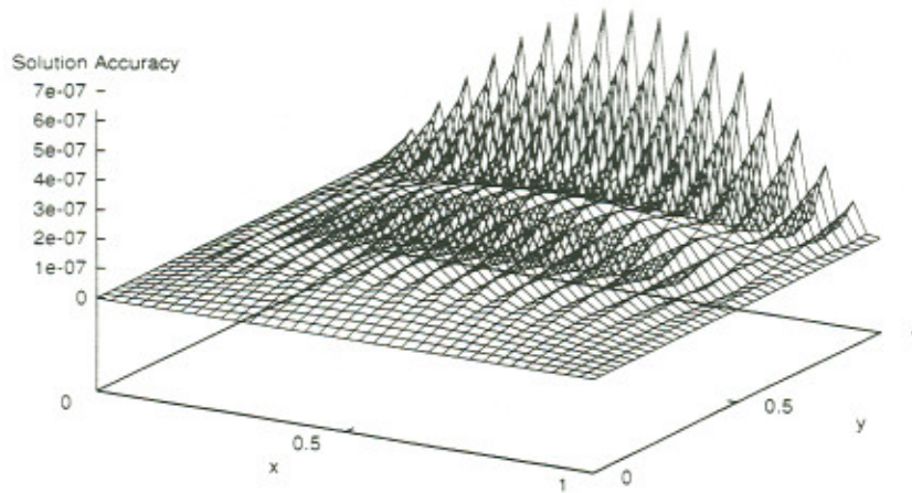
Figure 20: Problem 7: Accuracy of the FEM solution at the training points.
