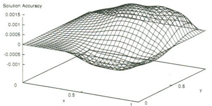
Figure 12: Problem 6: Accuracy of the computed solution at the test points.
