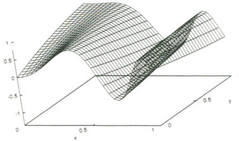
Figure 10: Exact solution of PDE problem 6.
