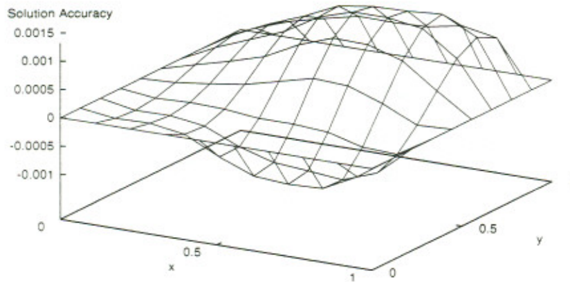
Figure 11: Problem 6: Accuracy of the computed solution at the training points.
