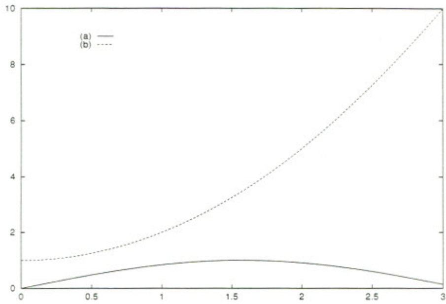
Figure 5: Exact solutions of the system of coupled ODEs.
