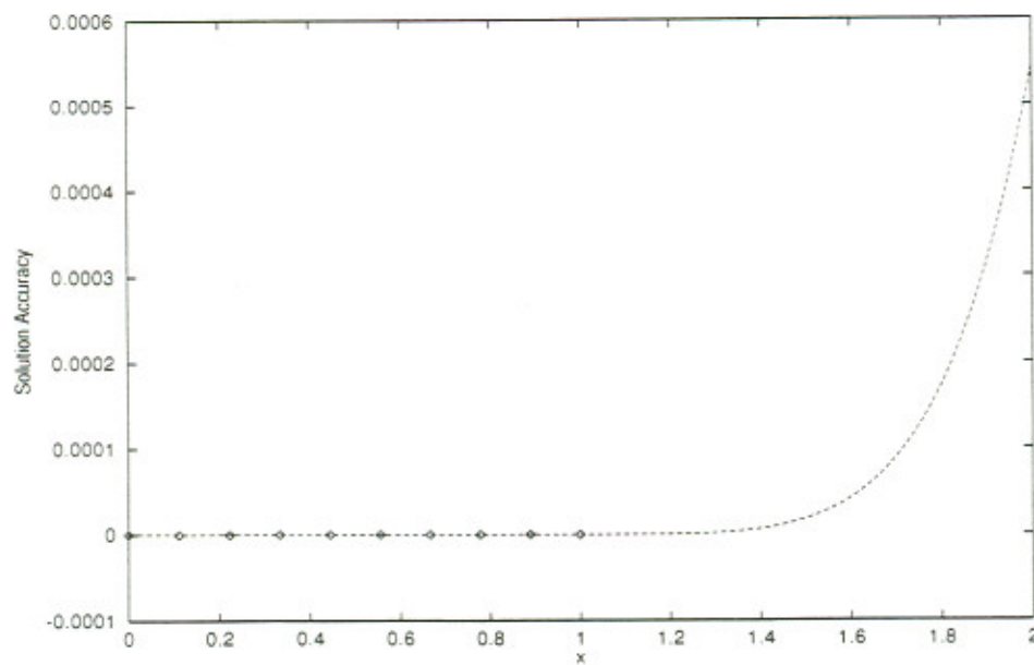
Figure 4: Problem 3 with boundary conditions: Accuracy of the computed solution.
