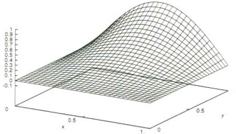
Figure 13: Exact solution of PDE problems 7 and 8.
