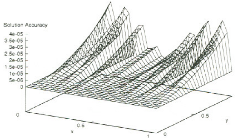
Figure 21: Problem 7: Accuracy of the FEM solution at the test points.
