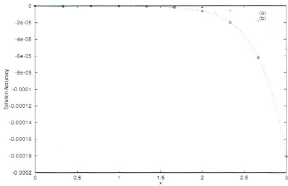
Figure 6: Problem 4: Accuracy of the computed solutions.
