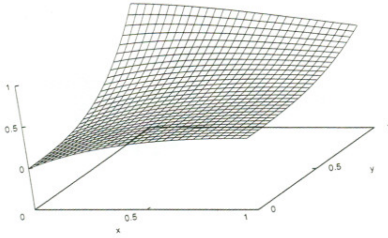
Figure 7: Exact solution of PDE problem 5.
