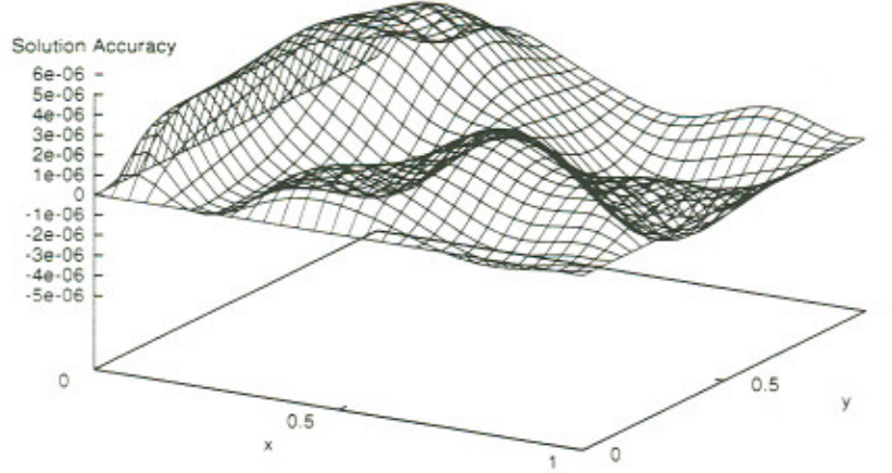
Figure 15: Problem 7: Accuracy of the computed solution at the test points.
