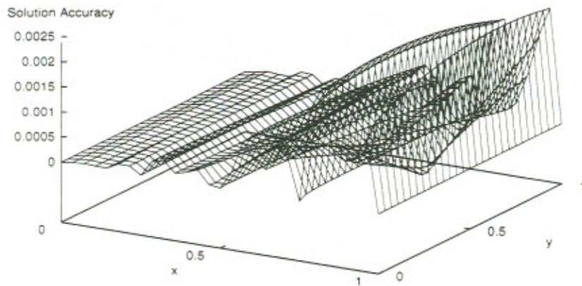
Figure 19: Problem 6: Accuracy of the FEM solution at the test points.
