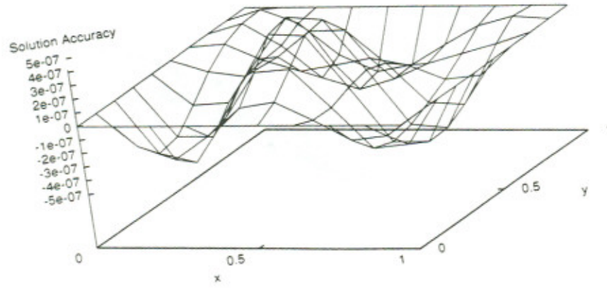
Figure 8: Problem 5: Accuracy of the computed solution at the training points.
