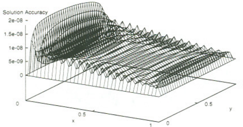
Figure 16: Problem 5: Accuracy of the FEM solution at the training points.
