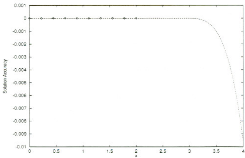
Figure 2: Problem 2: Accuracy of the computed solution.
