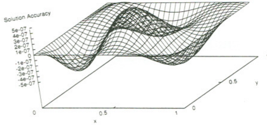
Figure 9: Problem 5: Accuracy of the computed solution at the test points.
