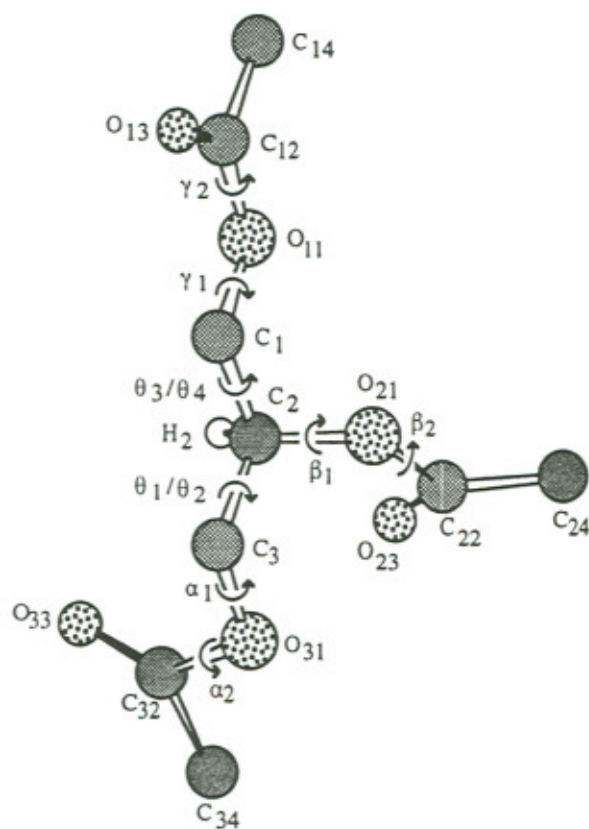
Fig. 1. The lowest triacetin conformer. Except for the mid-carbon hydrogen, the others are omitted for the sake of clarity.
