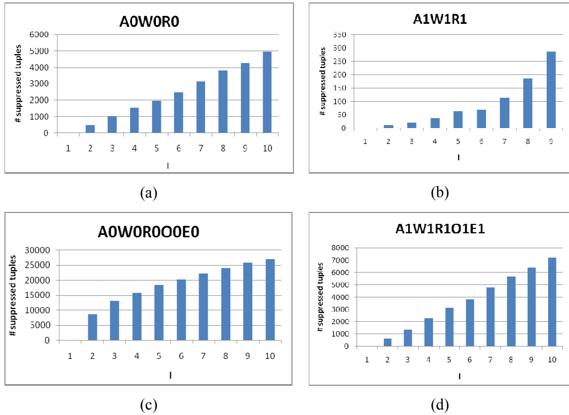
Figure 3.24 Cumulative histogram \gamma_{\alpha} l-diversity
