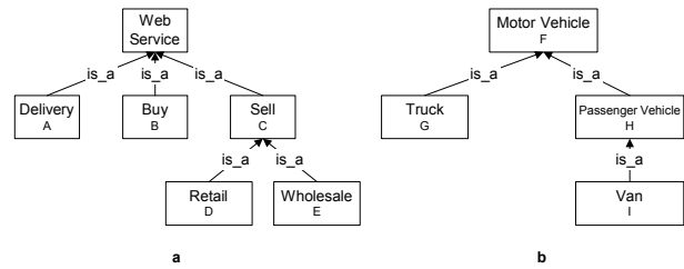
Figure 7. Service ontology and domain ontology
