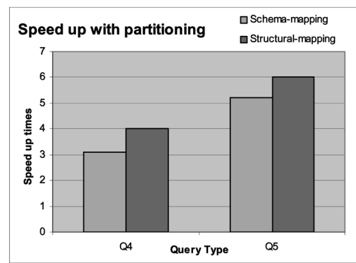
Fig. 17. Speed up ratios for Q4 and Q5.
