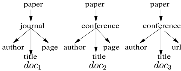
Fig. 10. S-graph-based similarity.
