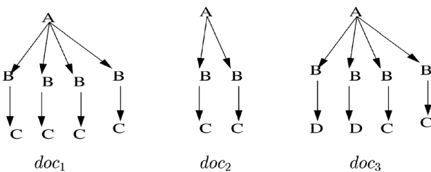
Fig. 7. Tree distances between documents.
