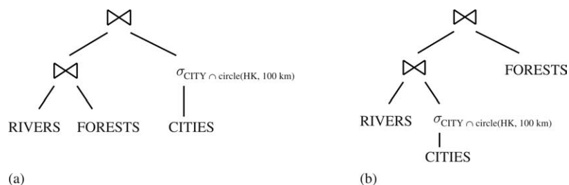
Figure 1. Two evaluation plans for a complex spatial query.
