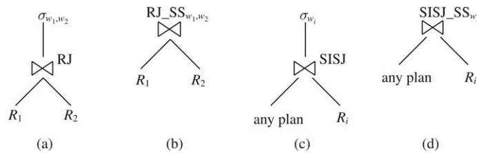
Figure 19. Combining selections with joins is always more efficient than evaluating them after the joins.
