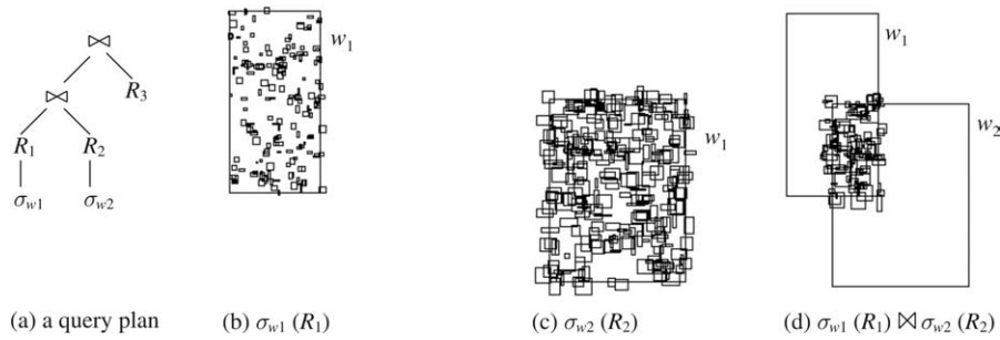
Figure 2. Example dependency between spatial operators.
