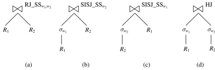
Figure 20. The four plans of \sigma_{w_1}(R_1) \bowtie \sigma_{w_2}(R_2) .
