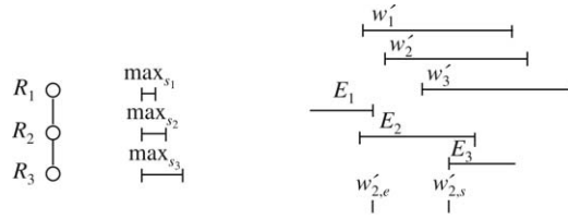
Figure 17. A qualifying triple of entries defining an invalid window at the next level.
