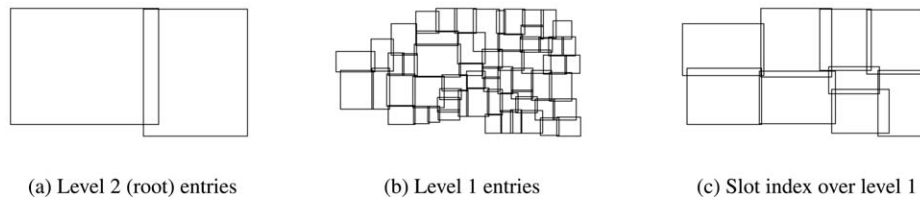
Figure 6. An R-tree and a slot index built over it.
