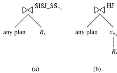
Figure 21. A case where SISJ_SS is always more efficient than HJ.
