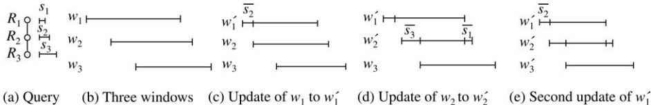
Figure 9. Selection window update propagation in a network of joined datasets.
