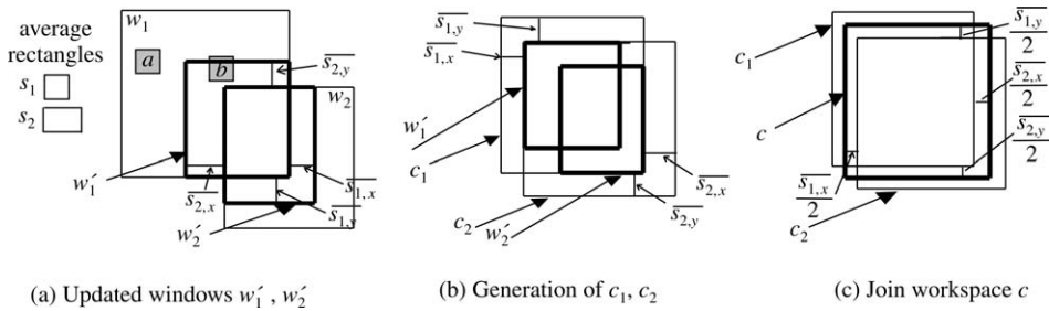
Figure 7. Generation of the join workspace.
