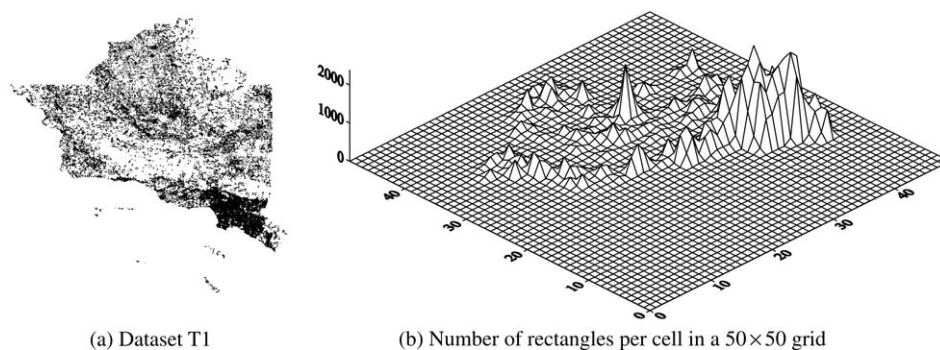
Figure 11. Skew in real dataset T1.
