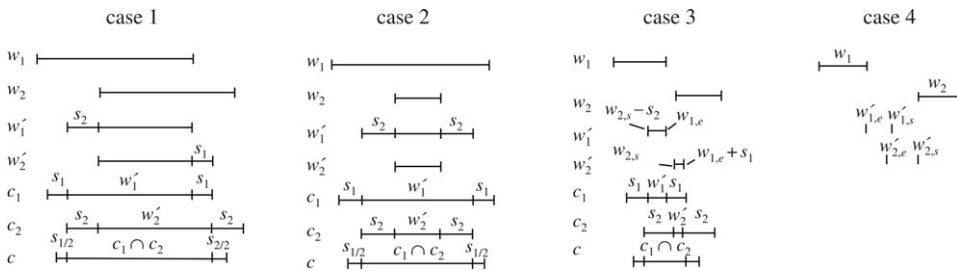
Figure 8. Windows that define the selectivity of a complex pairwise join.
