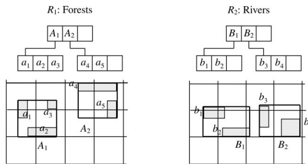
Figure 4. Two spatial datasets indexed by R-trees.
