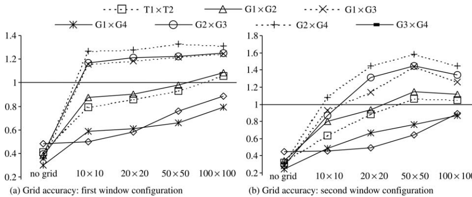
Figure 14. Accuracy of grids for various joins.
