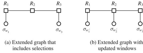
Figure 15. Graphs for the complex query \sigma_{w_1}(R_1) \bowtie R_2 \bowtie \sigma_{w_3}(R_3) .
