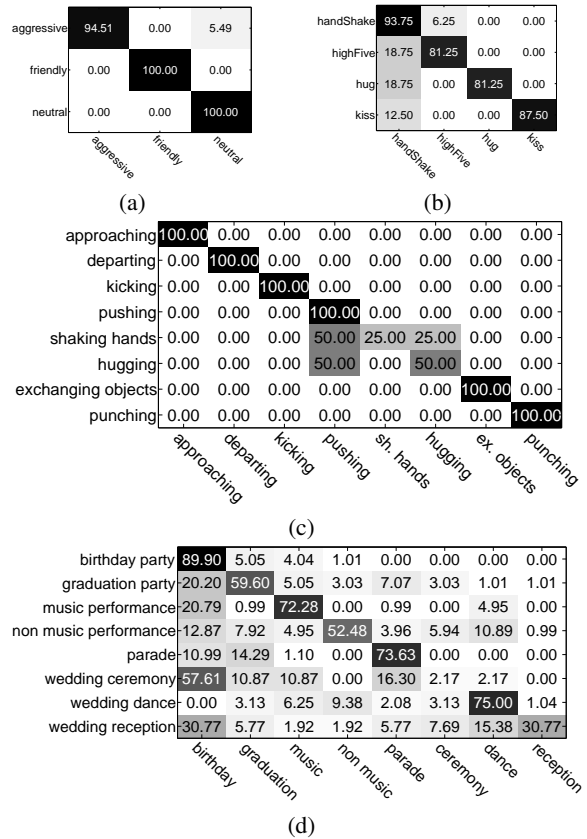
Fig. 3. Confusion matrices for the classification results for the best split of the proposed a-HCRF+ (entropy) variant for (a) the Parliament [23], (b) the TVHI [24], (c) the TPI [25], and (d) the USAA [26] datasets.
