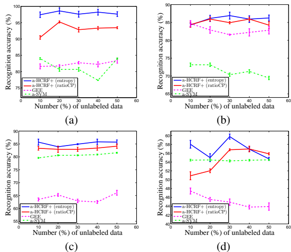
Fig. 2. Comparison of classification accuracies with respect to the number of unlabeled data for (a) the Parliament [23], (b) the TVHI [24], (c) the TPI [25], and (d) the USAA [26] datasets.
