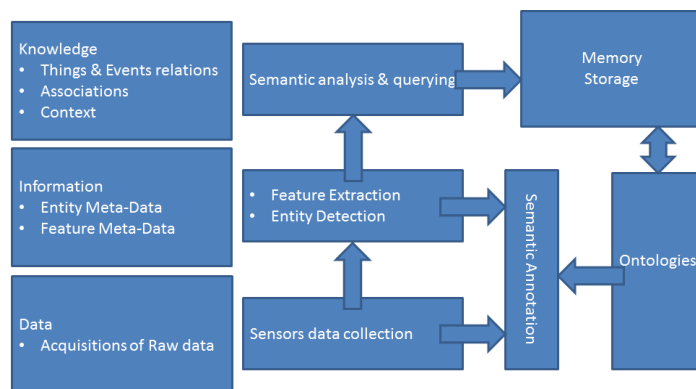
Figure-2.18. The generic data-to-knowledge architectural building blocks.
