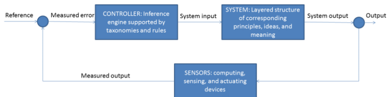
Figure-3.9 Context-awareness control by a first-order feedback loop.
