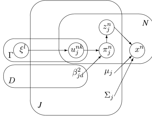
Fig. 3. Graphical model for the binary line process edge preserving model. Superscripts n, k \in [1, N] denotes pixel index, subscript j \in [1, J] denotes kernel (segment) index, d \in [1, D] describes the neighborhood direction type and l \in [1, \Gamma] denotes neighbor index.
