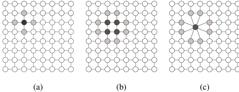
Fig. 11. Grid-scan updates on an example lattice with 8x8 elements and 1 st order neighborhoods. Black color shows the elements whose contextual mixing proportions need to be updated. Gray color shows their neighboring pixels. (a) Single element to be optimized and its neighbors. (b) Elements to be co-optimized by a step of grid scan and their neighbors. (c) The same elements to be co-optimized redrawn as one.
