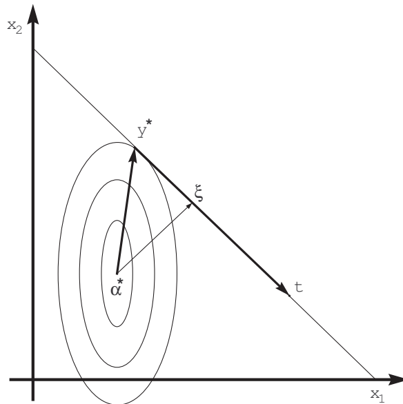
Fig. 6. Example projection to the constraints plane, in the two-dimensional case J = 2 . Ellipses represent contours of the quadratic approximation to the objective function; the line joining the x_1 and x_2 axes is the linear constraints plane, here x_1 + x_2 = 1, x_1, x_2 \geq 0 . The unconstrained maximizer is \alpha^* , the constrained maximizer is y^* and t is a point on the constraints plane. Point \xi shows the location of the solution proposed in [17].
