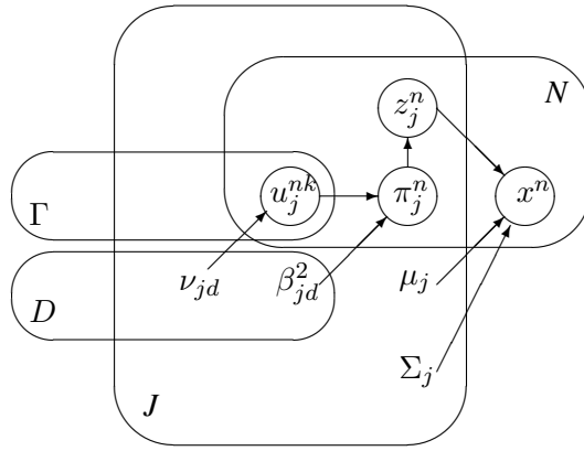
Fig. 4. Graphical model for the continuous line-process edge preserving model. Superscripts n, k \in [1, N] denotes pixel index, subscript j \in [1, J] denotes kernel (segment) index, d \in [1, D] describes the neighborhood direction type. \Gamma equals the maximum number of possible neighbors.
