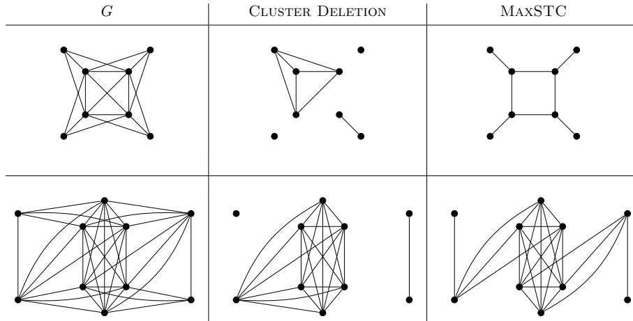
Fig. 2. Two examples of graphs with their corresponding optimal solutions for CLUSTER DELETION and MAXSTC, respectively. For the MAXSTC problem the edges of G that are not drawn in the solution correspond to the weak edges.
