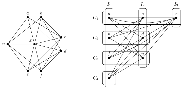
Fig. 1. A cograph and its greedy canonical partition (\mathcal{C}, \mathcal{I}) where \mathcal{C} = (C_1, C_2, C_3, C_4) and \mathcal{I} = (I_1, I_2, I_3) .
