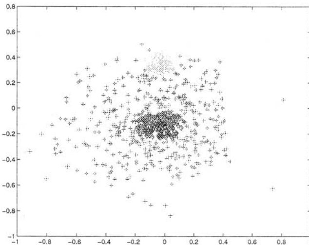
Fig. 4 Four-cluster partition of the Clouds data set using the greedy-EM algorithm
