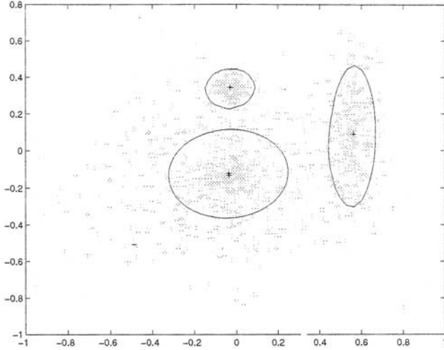
Fig. 3 Means and variances of the kernels using the greedy-EM algorithm for the Clouds data set
